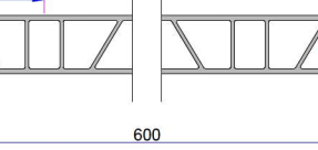
PVC Sill Profile (600mm) P.DNZ.01.60.E.600.19
