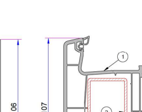
1. Eco Mullion Profile P.A.750.3006.600.0.BC.01 2. Reinforcement (26x30) 1,2mm - 34022 - 12115 1,5mm - 34022 - 15115 2 mm - 34022 - 20115
