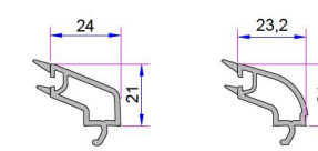
24mm Double Glazing Bead P.A.750.4200.600.0.HC
