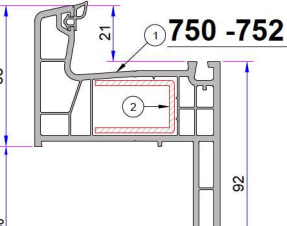
1. Frame Profile with 60mm Sill P.A.750.1919 2. Reinforcement (30x20x30) 1,2mm - 34022 - 12006 1,5mm - 34022 - 15006 2 mm - 34022 - 20006
