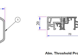
Alm. Threshold Profile AD16-089
