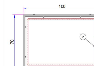
1. Box Profile (70x100) P.A.070.5202.600.0.00.19 2. Reinforcement (60x90) 1,2mm - 34022 - 12121 1,5mm - 34022 - 15121 2 mm - 34022 - 20121
