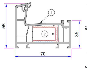
1. Eko Frame Profile P.A.750.1003.600.0.BC.01 2. Reinforcement (30x20x30) 1,2mm - 34022 - 12006 1,5mm - 34022 - 15006 2 mm - 34022 - 20006
