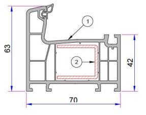
1. Frame Profile P.A.750.1000.600.0.BC.01 2. Reinforcement (30x25x30) 1,2mm - 34022 - 12004 1,5mm - 34022 - 15004 2 mm - 34022 - 20004
