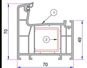
1. Super Frame Profile P.A.750.1001.600.0.BC.01 2. Reinforcement (29x30x29) 1,2mm - 34022 - 12002 1,5mm - 34022 - 15002 2 mm - 34022 - 20002
