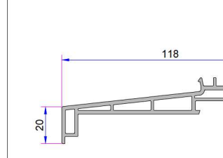
42mm Triple Glazing Bead P.A.532.4500.600.0.HC
