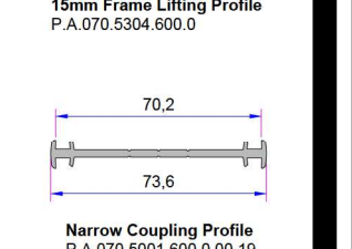
Frame Montage Profile P.A.060.5301.600.0.00.19
