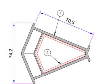
1. 135° Corner Profile P.A.070.5102.600.0.00.19 2. Reinforcement (25x55) 1,2mm - 34022 - 12303 1,5mm - 34022 - 15303 2 mm - 34022 - 20303
