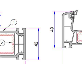
1. Outward Opening Sash Profile P.A.750.2001.600.0.BC.01 2. Reinforcement (25x25x25) 1,2mm - 34022 - 12003 1,5mm - 34022 - 15003 2 mm - 34022 - 20003
