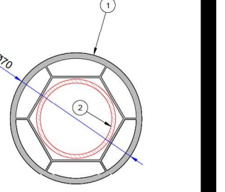
1. Angled Pipe Profile P.A.070.5106.600.0.00.19 2. Reinforcement (Ø42mm) 1,2mm - 34022 - 12502 1,5mm - 34022 - 15502 2 mm - 34022 - 20502
