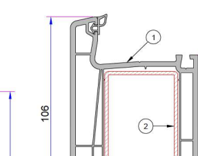
1. Super Static Mullion Profile P.A.750.3009.600.0.BC.01 2. Reinforcement (60x20) 1,2mm - 34022 - 12106 1,5mm - 34022 - 15106 2 mm - 34022 - 20106
