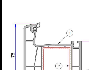
1. Mullion Profile P.A.750.3000.600.0.BC.01 2. Reinforcement (30x25x30) 1,2mm - 34022 - 12004 1,5mm - 34022 - 15004 2 mm - 34022 - 20004
