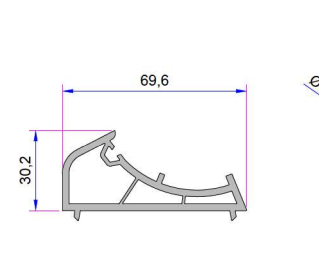
Angled Pipe Profile Adaptor P.A.070.5104.600.0.00.19
