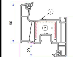
1. Sash Profile P.A.750.2000.600.0.BC.01 2. Reinforcement (25x30x25) 1,2mm - 34022 - 12025 1,5mm - 34022 - 15025 2 mm - 34022 - 20025
