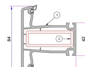
1. Offset Type Sash Profile P.A.750.2200.600.0.BC.01 2. Reinforcement (25x30x25) 1,2mm - 34022 - 12025 1,5mm - 34022 - 15025 2 mm - 34022 - 20025
