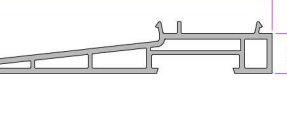
Sill Profile P.A.058.5504.600.0.00.19
