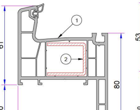
1. Frame Profile with Sill P.A.750.1200.600.0.BC.01 2. Reinforcement (30x25x30) 1,2mm - 34022 - 12004 1,5mm - 34022 - 15004 2 mm - 34022 - 20004
