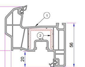
1. Offset Type Sash Profile (6 Chambered) P.A.750.2205.600.0.BC.01 2. Reinforcement (25x30x25) 1,2mm - 34022 - 12025 1,5mm - 34022 - 15025 2 mm - 34022 - 20025
