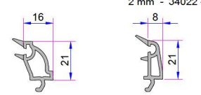
32mm Triple Glazing Bead P.A.101.4202.600.0.HC
