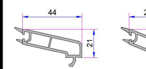
4-6mm Single Glazing Bead P.A.750.4000.600.0.HC
