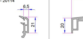
40mm Triple Glazing Bead P.A.532.4400.600.0.HC
