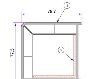
1. 90° Corner Profile P.A.070.5100.600.0.00.19 2. Reinforcement (55x55) 1,2mm - 34022 - 12305 1,5mm - 34022 - 15305 2 mm - 34022 - 20305
