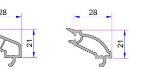
20mm Double Glazing Bead P.A.750.4100.600.0.HC
