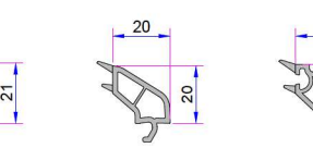
24mm Double Glazing Bead P.A.750.4204.600.0.HC
