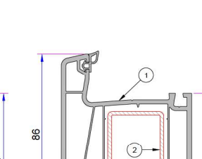
1. Static Mullion Profile P.A.750.3007.600.0.BC.01 2. Reinforcement (40x20) 1,2mm - 34022 - 12114 1,5mm - 34022 - 15114 2 mm - 34022 - 20114
