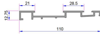
Aluminium Threshold Second Sash Rail AD16-025
