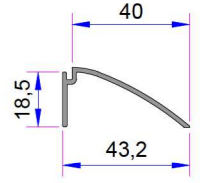
20mm Threshold Inner Profile AD16-080
