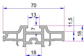
Hebeschiebe Sash and RailAdaptor P.A.930.6500.600
