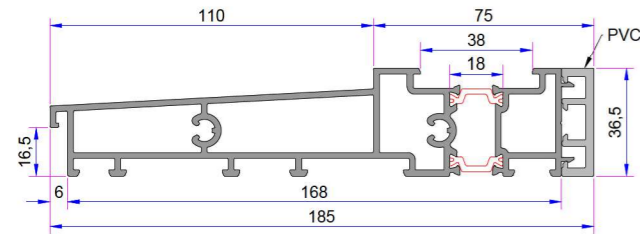
Hebeschiebe Interior Part PVC Thermo Insulation Aluminium Threshold AD16-026
