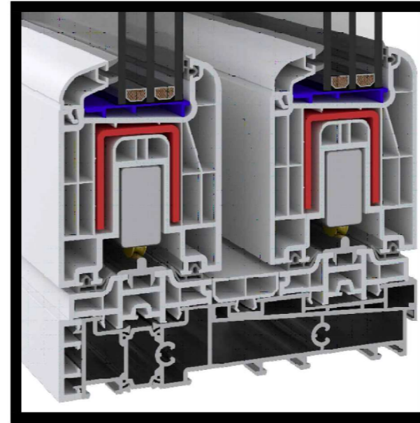
Hebeschiebe Frame Middle Adaptor P.A.900.6503.600
