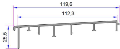
Hebeschiebe Aluminium Threshold Cover AD16-024
