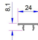
Second Threshold Rail Cover AD16-082
