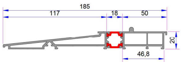
Hebeschiebe Aluminium Threshold with Thermo Insulation 20mm AD16-079
