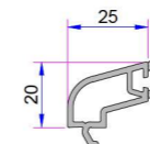
Triple Glazing Bead (32mm) P.A.800.4500.600.0.HC
