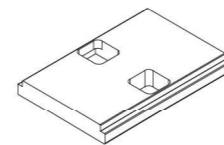
PVC Ve Alm. LowerFrame Corner Connection 21238.0000.0
