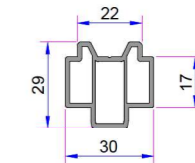
Stable Guide For Sash Aluminium AD16-021
