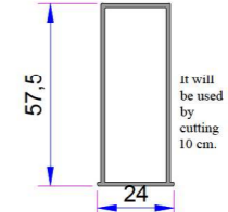
20mm'lik Alm. Sash Bedding AD16-083
