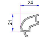
Triple Glazing Bead (32mm) P.A.750.4204.600.0.HC
