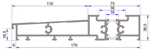
Hebeschiebe Aluminium Threshold with Thermo Insulation AD16-027
