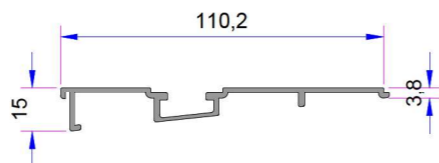
Aluminium Threshold Second Sash Rail AD16-081
