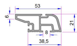
Hebeschiebe Sash Lap Strip Profile P.A.930.6504.600
