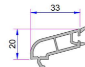
Double Glazing Bead (24mm) P.A.800.4200.600.0.HC
