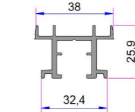
Frame Top Rail Aluminium AD16-019
