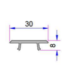
Fly-Screen Sash Cover P.A.242.5701.600
