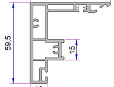
Alum. Sliding Mullion with Three Chambered AD16060
