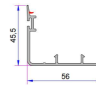
PVC Sash Cover Profile P.A.232.5709.600.0.00.01
