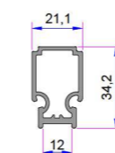
Alm. Double Rail Adaptor Profile AD16011
