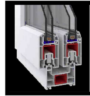
PVC Sash Cover Profile P.A.232.5701.650.0.00.19
