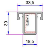
Fly-Screen Mullion Profile P.A.242.3200.600.0.00.01
