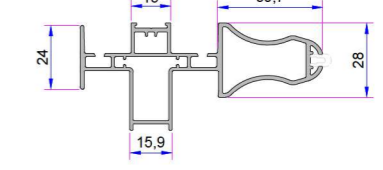
With Alum. Grillage Double Sash Middle Adaptor AD16059
