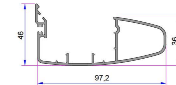
Alm. Sash Cover Grillage Profile 16028.601.5.2.0.9016
