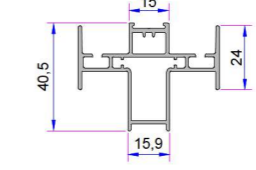
With Alum. Lug Double Sash Middle Adaptor AD16058
