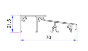
Aluminium Threshold Profile AD16-002
