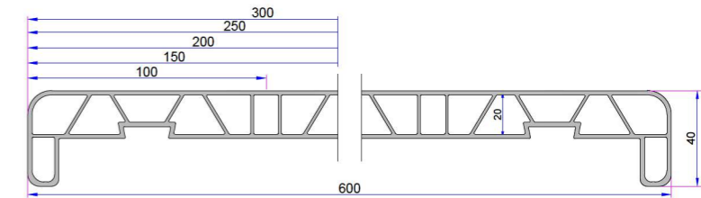
PVC Sill Profile (600mm) P.DNZ.01.60.E.600.19
