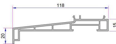
Sill Profile P.A.058.5504.600.0.00.19
