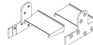
Aluminium Threshold Wedge 221013.0000.L - 221013.0000.R
