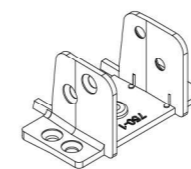
Mullion Connector 34007-12140
