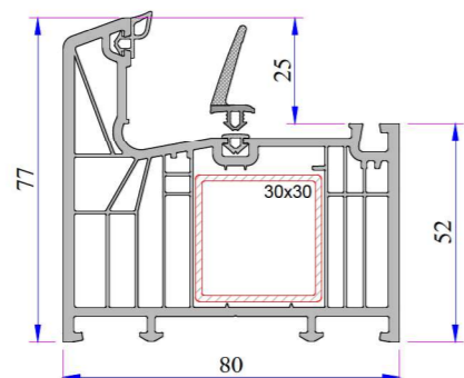
Super Frame Profile P.A.883.1001.600.2.BC.01 Reinforcement (30x30)
