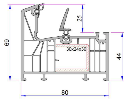
Frame Profile P.A.883.1000.600.2.BC.01 Reinforcement (30x24x30)
