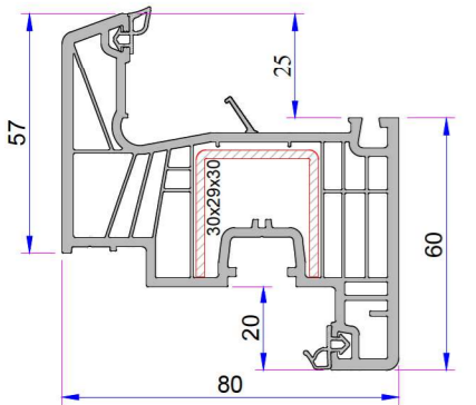
Sash Profile P.A.883.2000.600.2.BC.01 Reinforcement (30x29x30)
