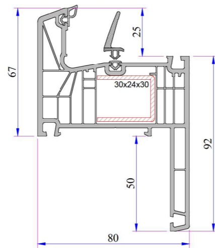
Frame Profile with Sill P.A.883.1200.600.2.BC.01 Reinforcement (30x24x30)
