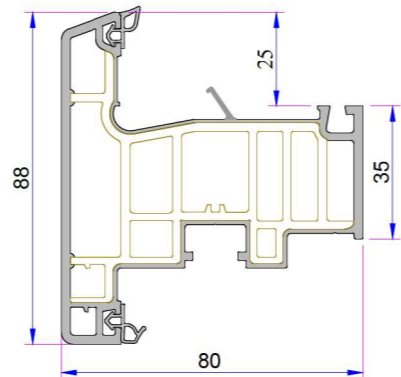
Outward Opening Sash Profile P.A.883.2001.600.2.BC.01
